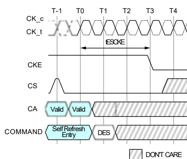
Figure 75 - tESCKE Timing
