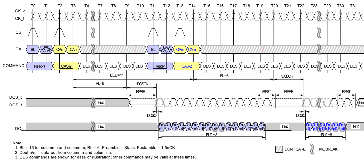
Figure 41 - Consecutive Reads Operation: tCCD = Min +3, Preamble = Static, 1.5nCK Postamble
