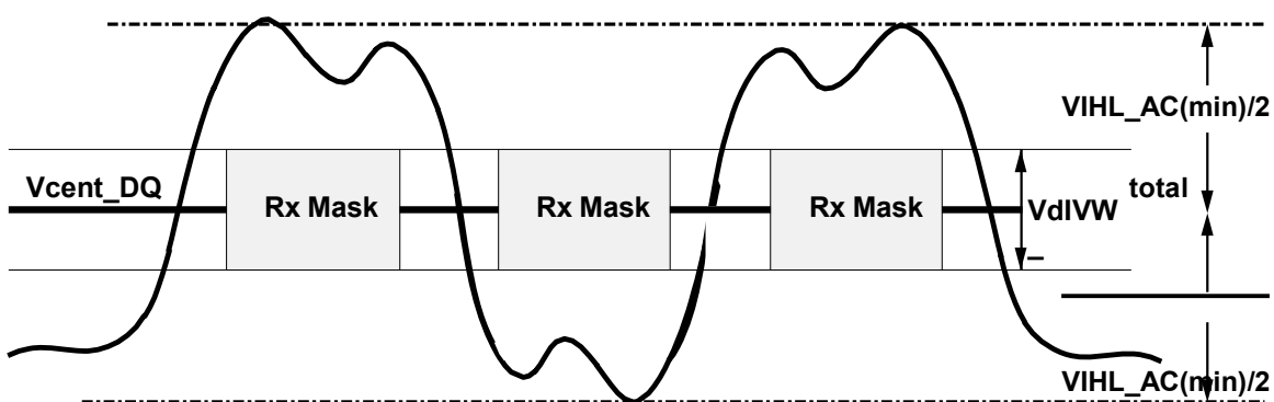
Figure 194 - DQ VIH_L_AC definition (for each input pulse)
