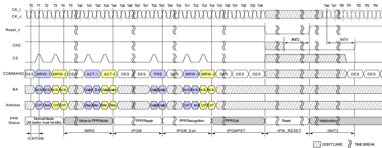
Figure 162 - PPR Timing
