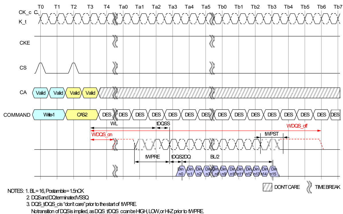
Figure 21 - DQS Write Preamble and Postamble: 1.5nCK Postamble
