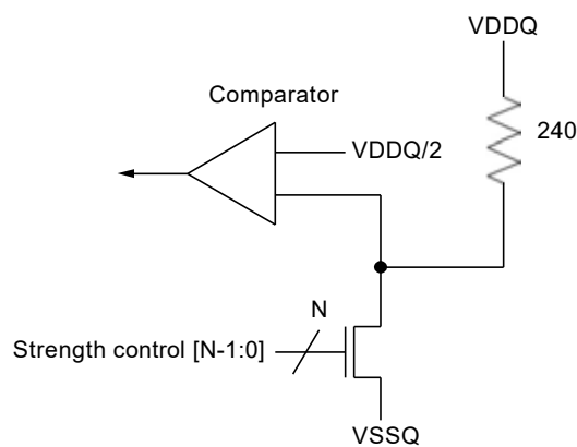
Figure 181 - Pull-down calibration
