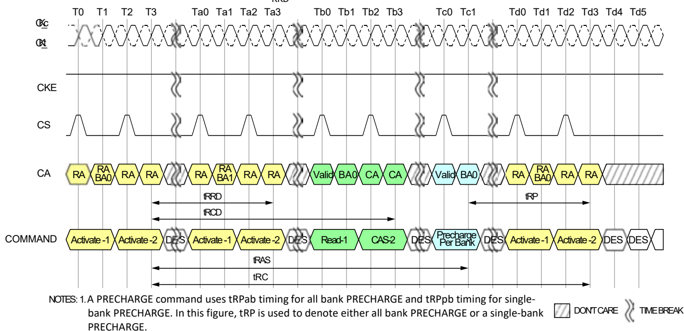
Figure 5 - Activate Command
