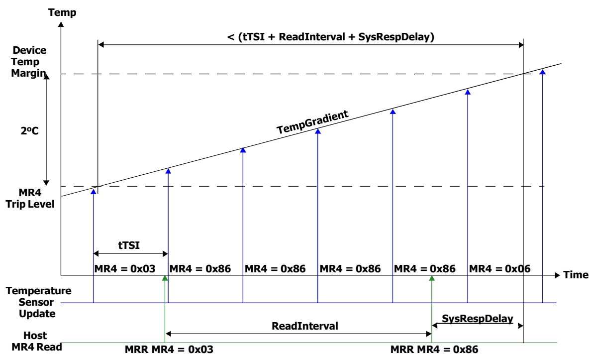
Figure 131 - Temp sensor Timing
