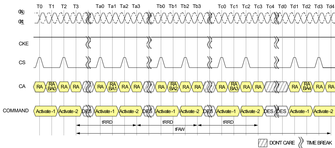
Figure 6 - tFAW Timing
