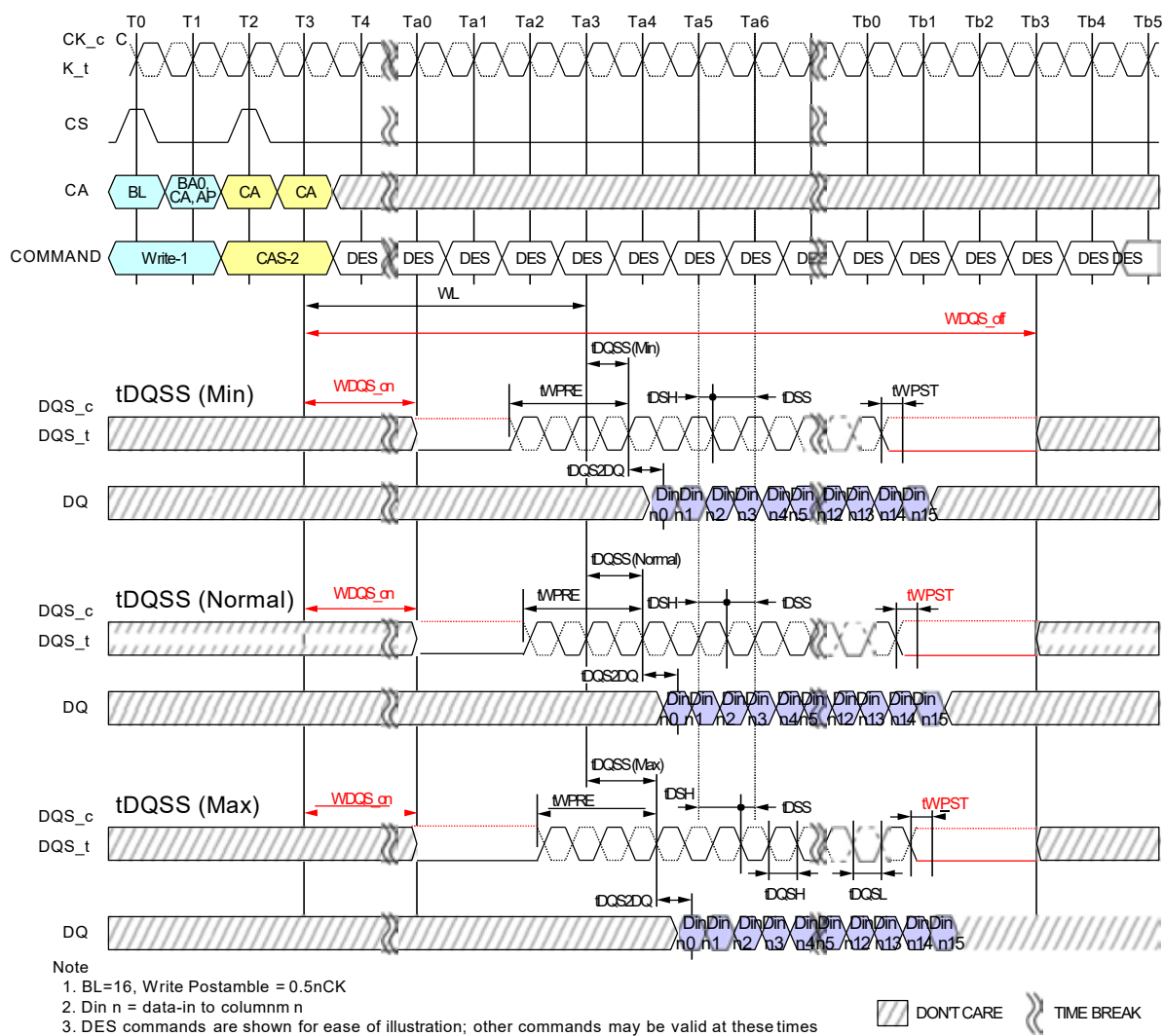
Figure 24 - Write Timing
