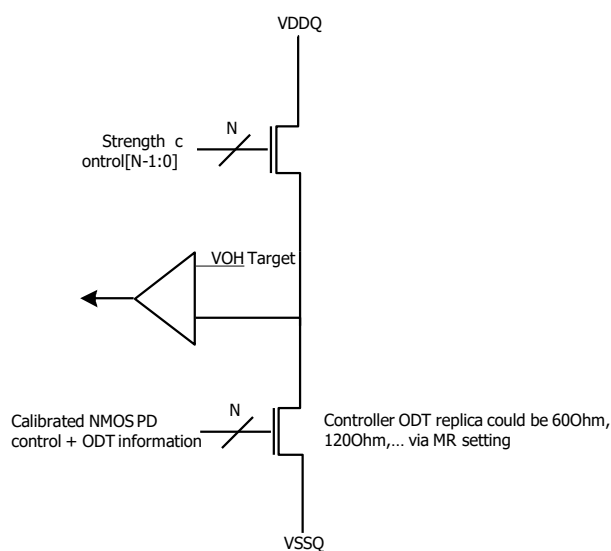
Figure 182 - Pull-up calibration
