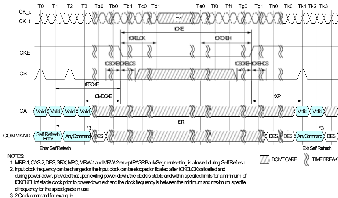
Figure 74 - Command input timings after Power Down Exit during Self Refresh
