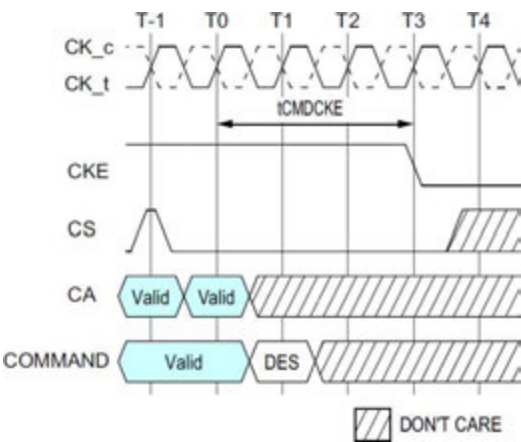
Figure 160 - tCMDCKE Timing
