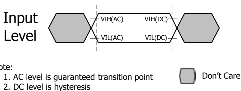
Figure 163 - Input AC timing definition for CKE
