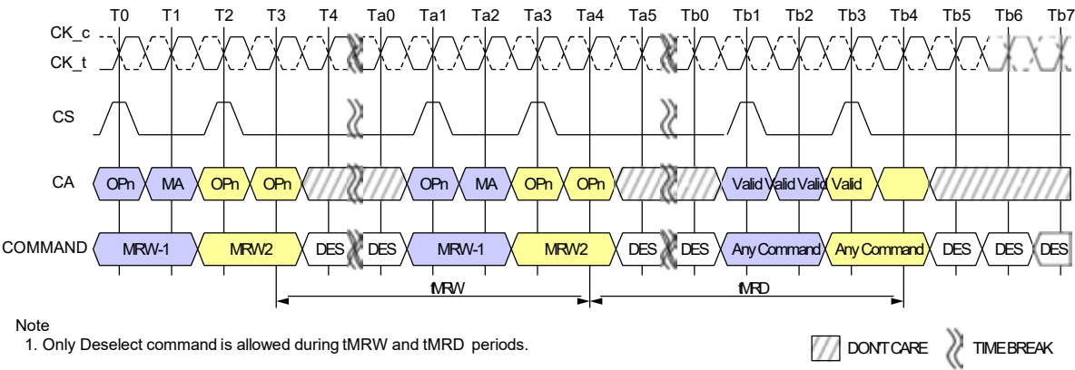
Figure 82 - Mode Register Write Timing
