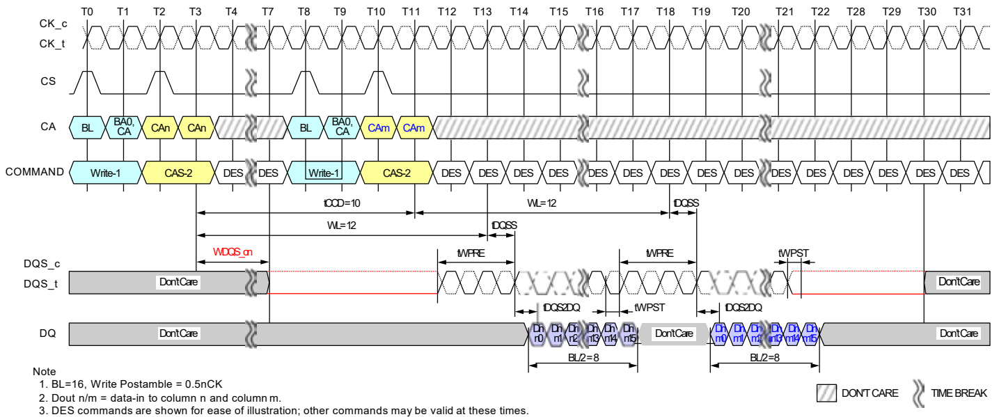
Figure 48 - Consecutive Writes Operation: t_{CCD} = \text{Min} + 2, 0.5nCK Postamble
