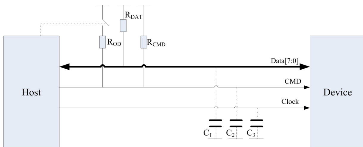
Figure 4 Bus Circuitry Diagram
